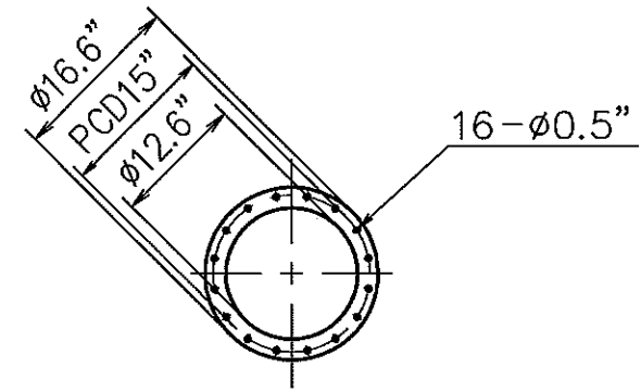
Suction & Discharge Flange
